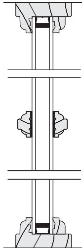
3/4" Insul 7/8" SDL
