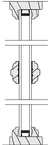
3/4" Insul 1-3/8" SDL
