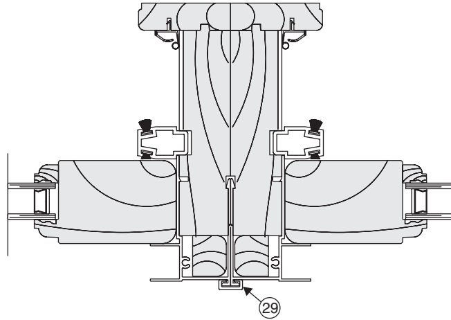
Vinyl TFT Vertical Mull
