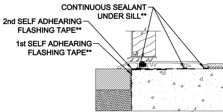
Vertical Section Detail - ADA Sill
